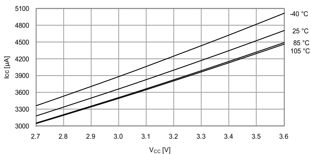
Figure 33-366. Idle Mode Current vs. V_{CC}
