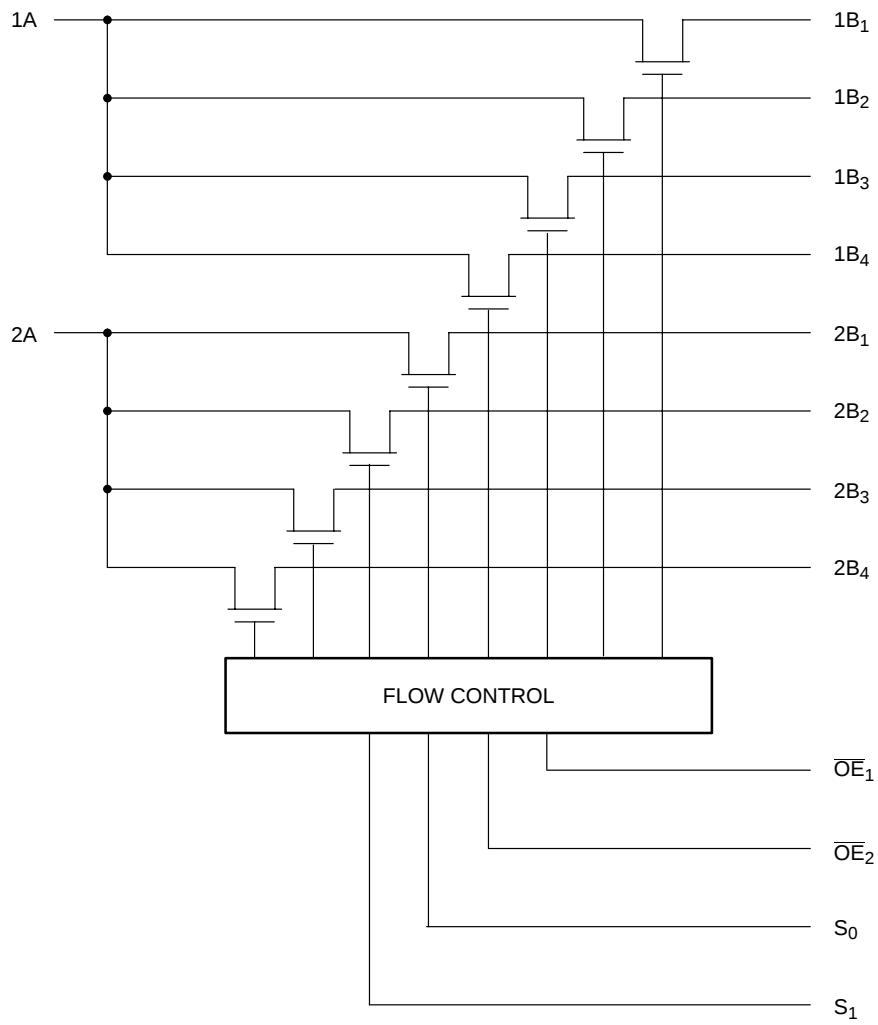
Figure 3. Logic Diagram
