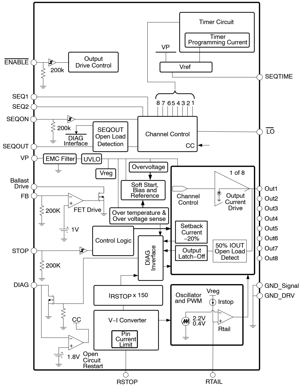
Figure 1. Block Diagram
