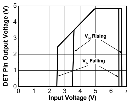
Figure 13. DET Pin Output Voltage vs Input Voltage R_{DET} = 470\Omega , I_{BAT} = 0mA , T_A = 25^\circ C
