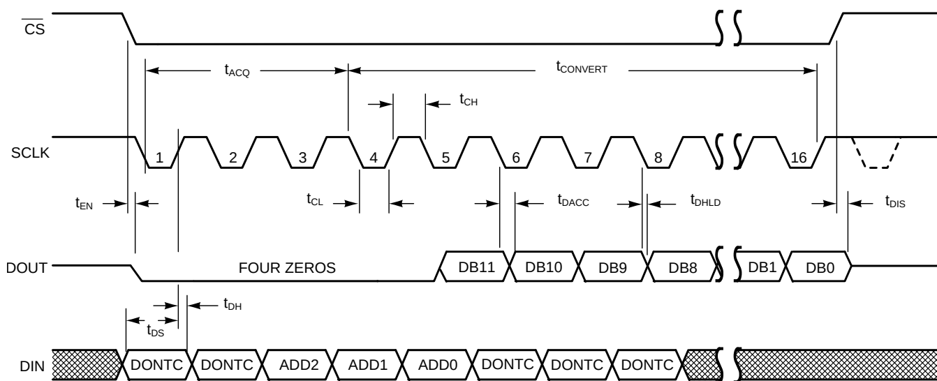
Figure 2. ADC128S102 Serial Timing Diagram
