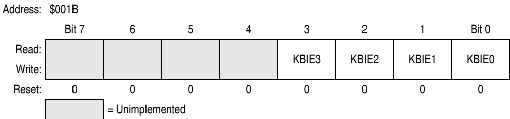
Figure 9-5. Keyboard Interrupt Enable Register (INTKBIER)
