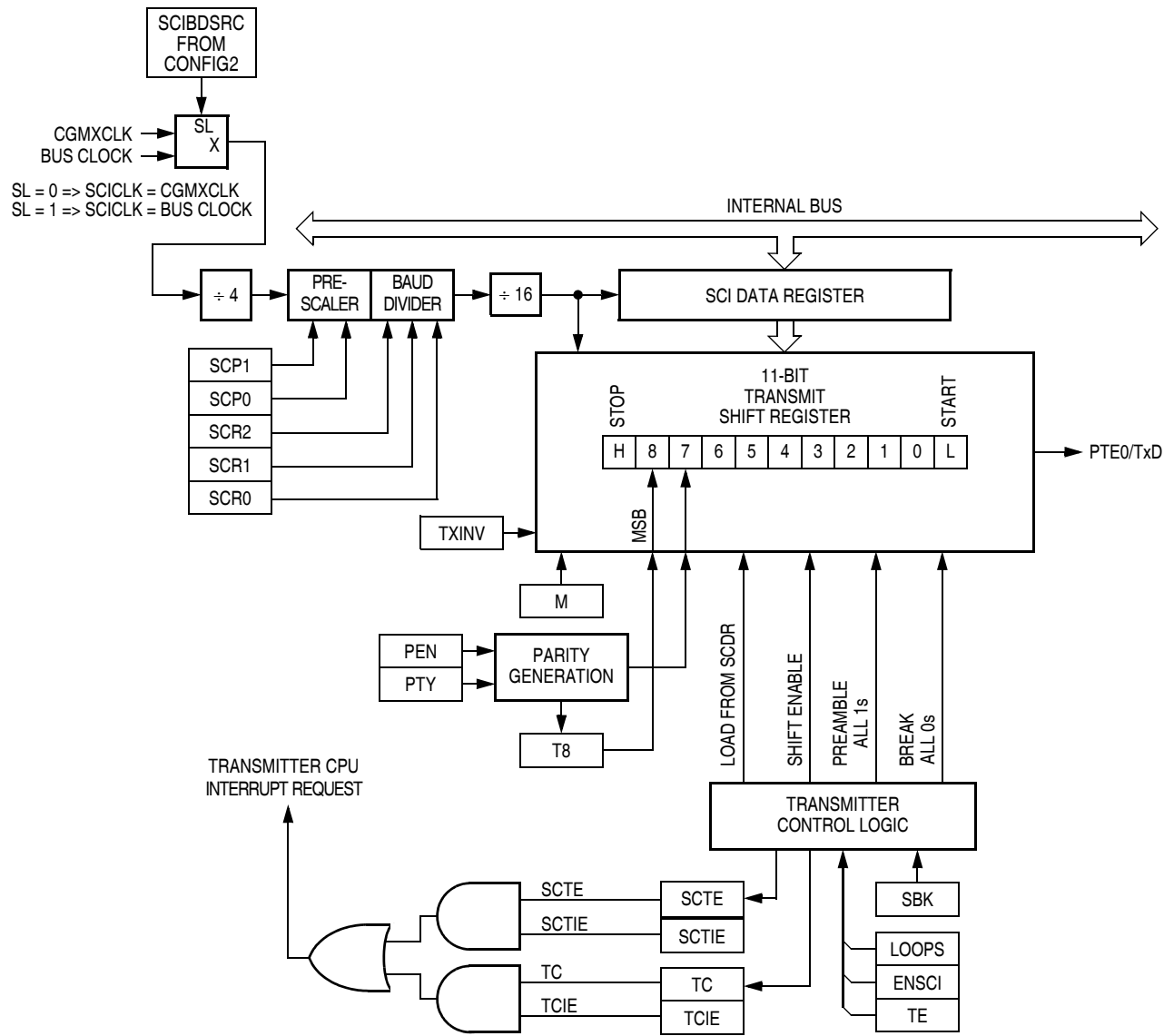
Figure 13-5. SCI Transmitter
