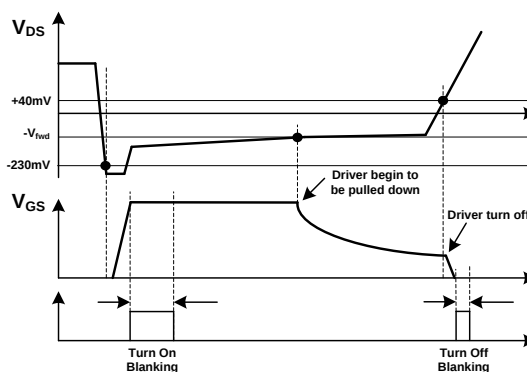
Figure 3: Turn-On/Off Timing Diagram
