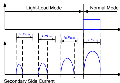
Figure 5: MP6924, MP6924A Exiting Light-Load Mode
