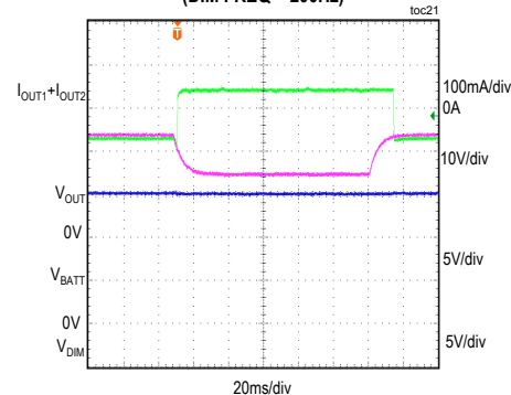
STARTUP WAVEFORM OF LED DRIVER WITH DIM DUTY = 25% (DIM FREQ = 200Hz)
