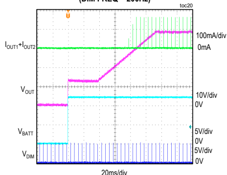
STARTUP WAVEFORM OF LED DRIVER WITH DIM PW = 25μs (DIM FREQ = 200Hz)
