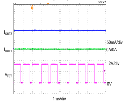
LED FAULT CREATED BY SHORTING 3 LEDs IN STRING1
