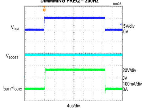
LED SWITCHING WITH DIMMING PULSE WIDTH OF 25μs DIMMING FREQ = 200Hz
