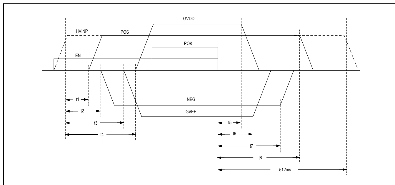
Figure 10. Sequencing Diagram
