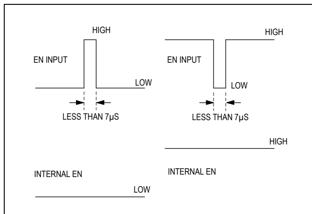
Figure 11. Power-Up/Power-Down Sequencing and Timing Waveform
