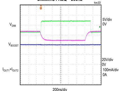
LED SWITCHING WITH DIMMING PULSE WIDTH OF 1μs DIMMING FREQ = 200Hz
