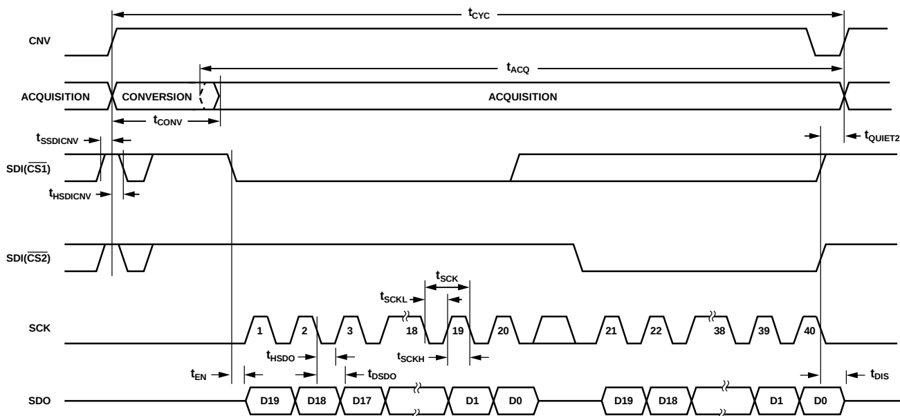
Figure 62. CS Mode, 4-Wire Without the Busy Indicator Serial Interface Timing Diagram (Status Bits Not Shown)
