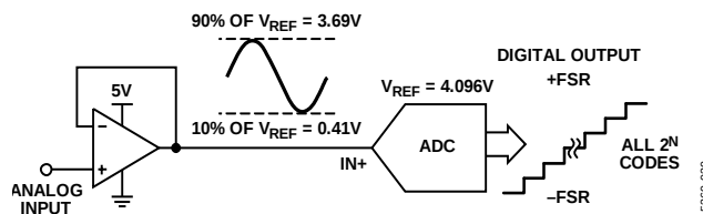
Figure 46. Span Compression
