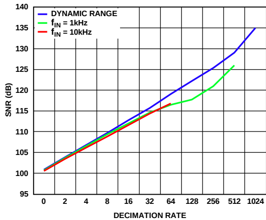
Figure 23. SNR vs. Decimation Rate for Various Input Frequencies, 1.8 MSPS
