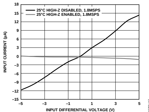
Figure 2. Input Current vs. Input Differential Voltage
