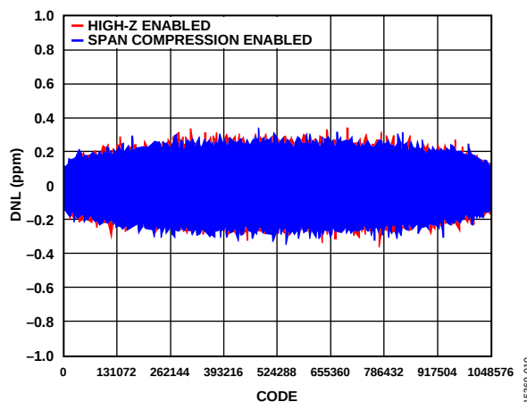
Figure 10. DNL vs. Code for High-Z and Span Compression Modes Enabled, V_{REF} = 5\text{ V}
