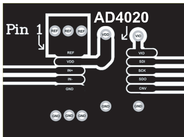
Figure 67. Example Layout of the AD4020 (Top Layer)
