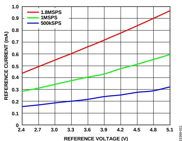
Figure 34. Reference Current vs. Reference Voltage
