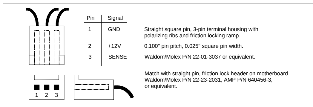
Figure 32. Boxed Processor Fan Heatsink Power Cable Connector Description
