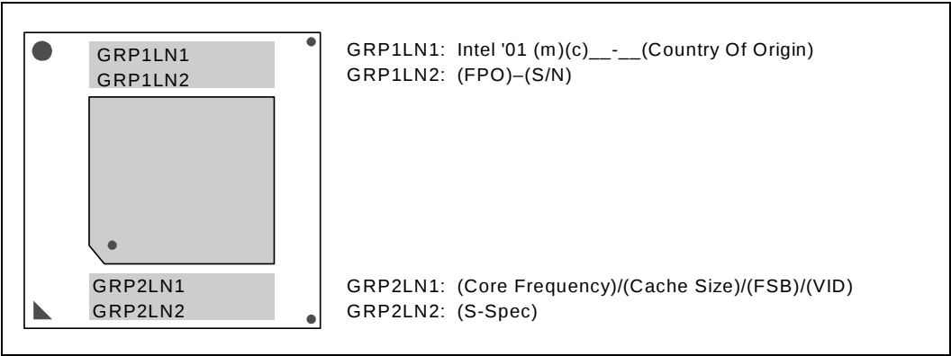
Figure 25. Top Side Processor Markings
