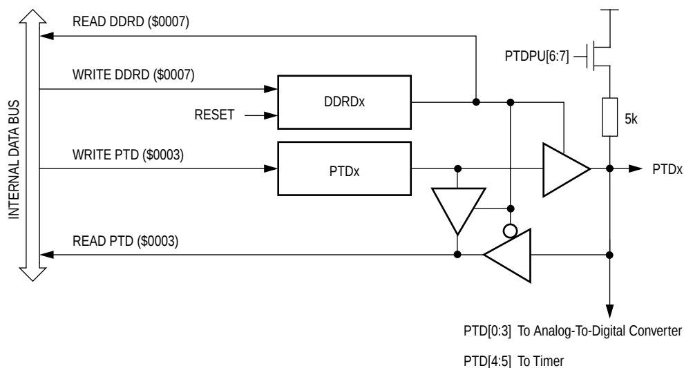
Figure 12-11. Port D I/O Circuit
