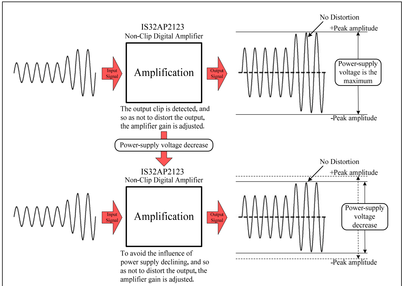
Figure 19 Operation Outline of AGC Control Function
