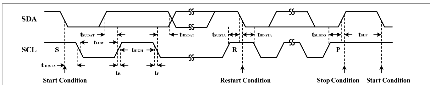
Figure 12 Interface Timing
