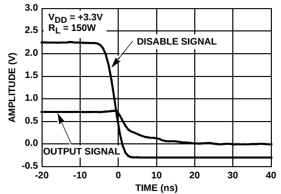
FIGURE 14. DISABLE TIME
