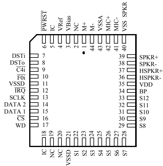
44 PIN PLCC
