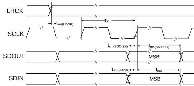
Figure 6. Serial Port Timing (Master Mode)
