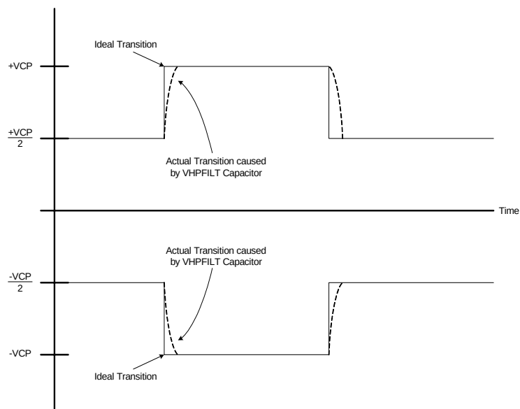
Figure 15. VHPFILT Transitions
