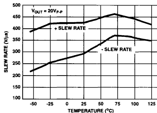
FIGURE 49. SLEW RATE vs TEMPERATURE
