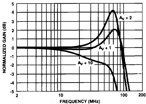
FIGURE 40. NON-INVERTING FREQUENCY RESPONSE
