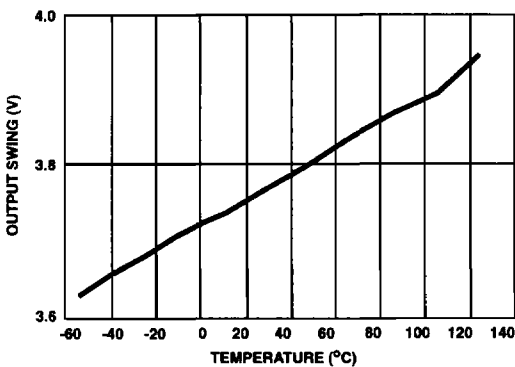
FIGURE 54. OUTPUT SWING vs TEMPERATURE
