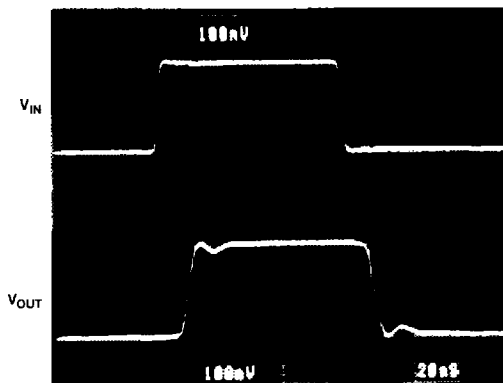
FIGURE 4. SMALL SIGNAL RESPONSE
