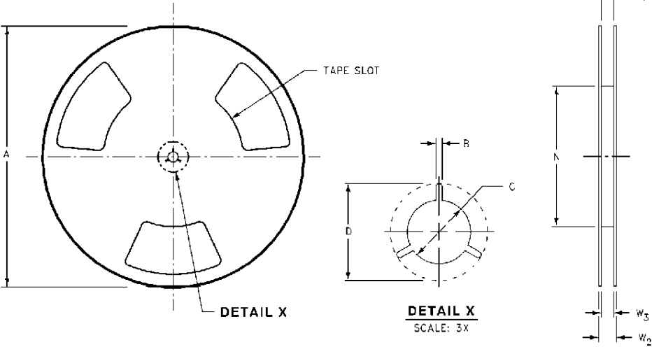
REEL DIMENSIONS inches (millimeters)
