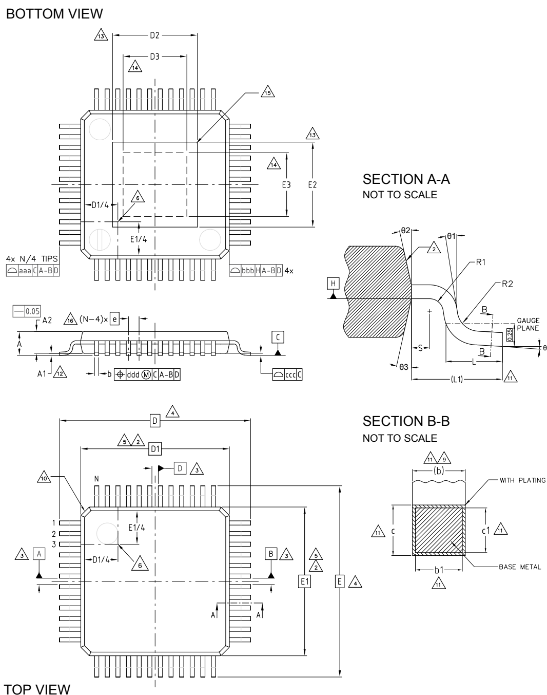
Figure 3. TQFP48 (7x7x1 mm exposed pad down) package outline
