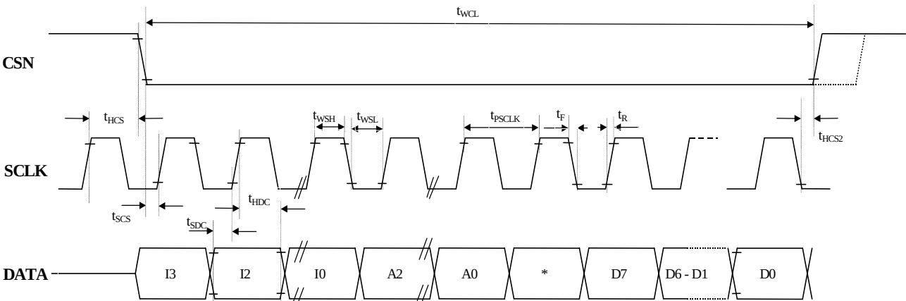
図 4 Serial Interface Timing < WRITE >
