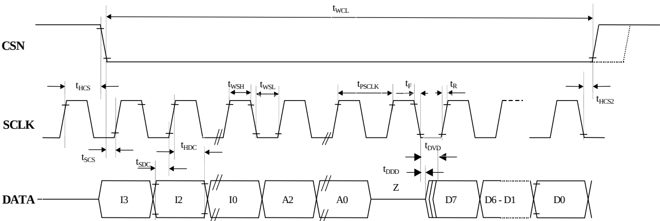
図 5 Serial Interface Timing < READ >
