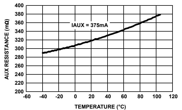
FIGURE 8. AUX r_{DS(ON)} vs TEMPERATURE
