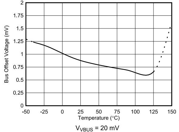
Figure 6-11. Bus Input Offset Voltage vs. Temperature
