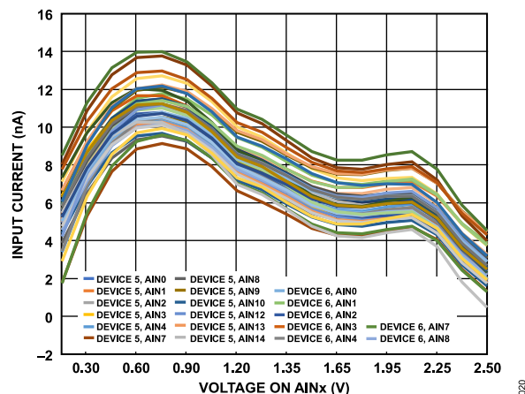
Figure 11. Input Current vs. Voltage on AINx, f_{\text{SAMPLE}} = 100 \text{ kSPS}
