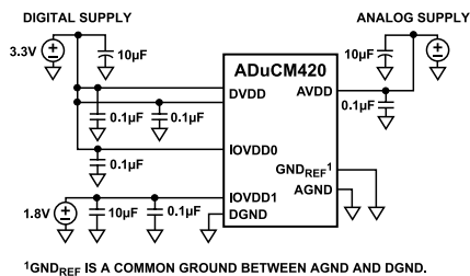
Figure 15. External Multiple Supply Connections
