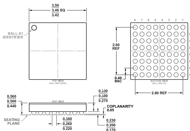
Figure 21. 64-Ball Wafer Level Chip Scale Package [WLCSP] (CB-64-2)
