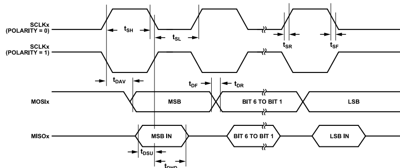
Figure 5. SPI Master Mode Timing (CPHA = 1)
