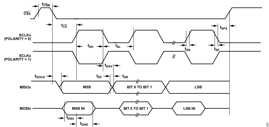
Figure 3. SPI Slave Mode Timing (Serial Clock Phase Mode, CTL Register, Bit 2, CPHA = 0)
