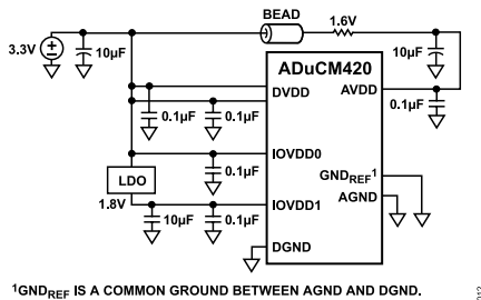
Figure 16. External Single-Supply Connections
