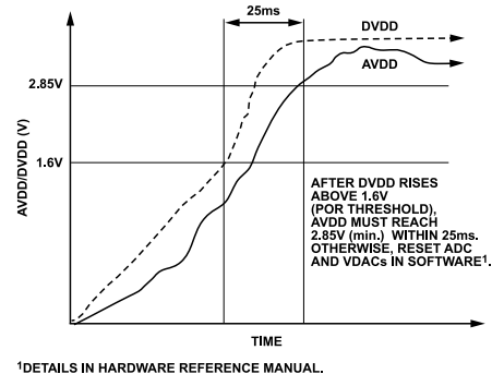
Figure 18. AVDD Power-Up Requirements
