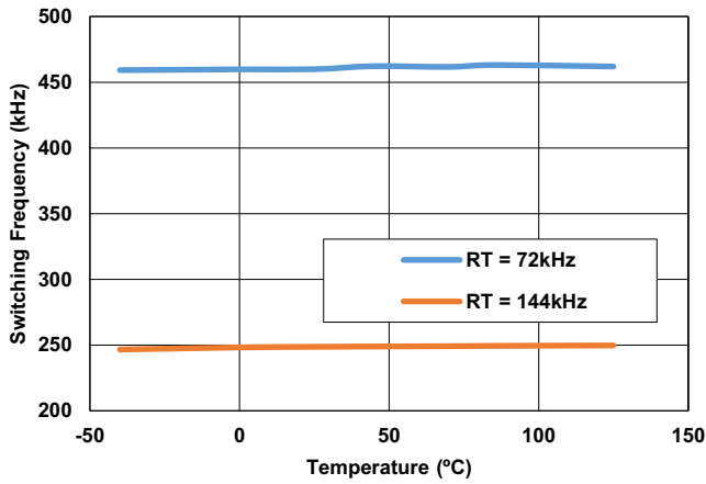
Figure 13. Switching Frequency vs Temperature
