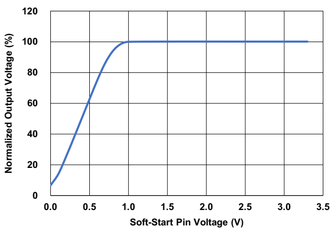
Figure 17. Normalized Output Voltage vs Voltage on Soft-Start Pin
