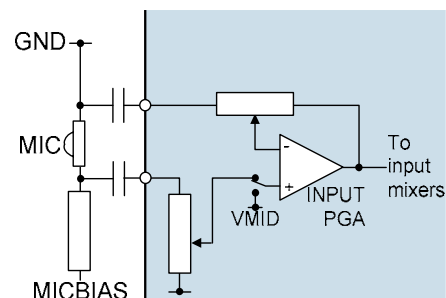
Figure 16 Differential Microphone Input
