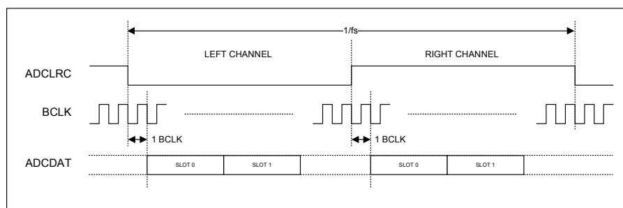
Figure 44 TDM in I 2 S Mode
