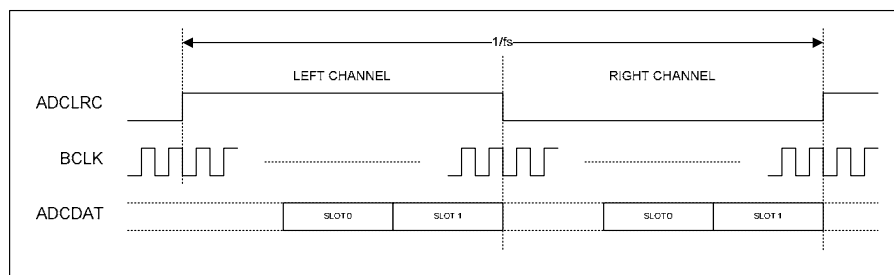
Figure 42 TDM in Right-Justified Mode
