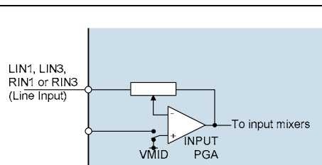
Figure 17 LIN1, RIN1, LIN3 or RIN3 as Line Inputs
