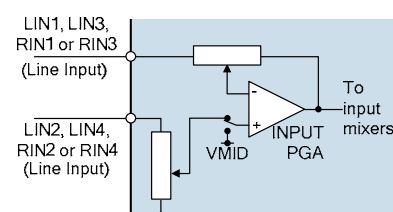
Figure 19 Differential Line Inputs
