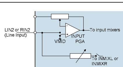
Figure 18 LIN2 or RIN2 as Line Inputs
