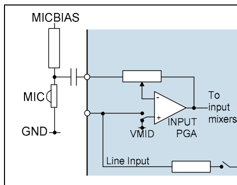
Figure 15 Single-Ended Microphone Input
