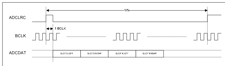
Figure 45 TDM in DSP Mode A
