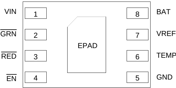
Figure 3. 34674 Pin Connections
