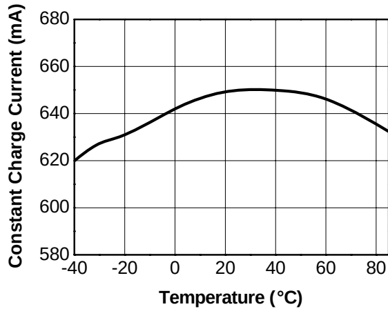
Figure 11. Constant Charge Current vs Temperature I_{CHG} = 650\text{ mA} , V_{IN} = 5.0\text{ V} , V_{BAT} = 3.9\text{ V}
