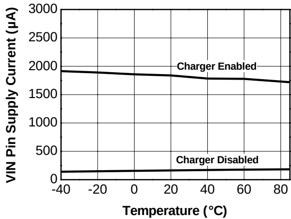
Figure 16. VIN Pin Supply Current vs Temperature I_{CHG} = 650 \text{ mA} , V_{BAT} = 5.0 \text{ V} , I_{BAT} = 0 \text{ mA}
