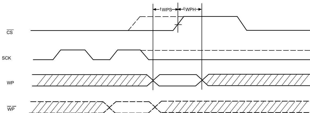
Figure 9. \overline{WP} Timing
