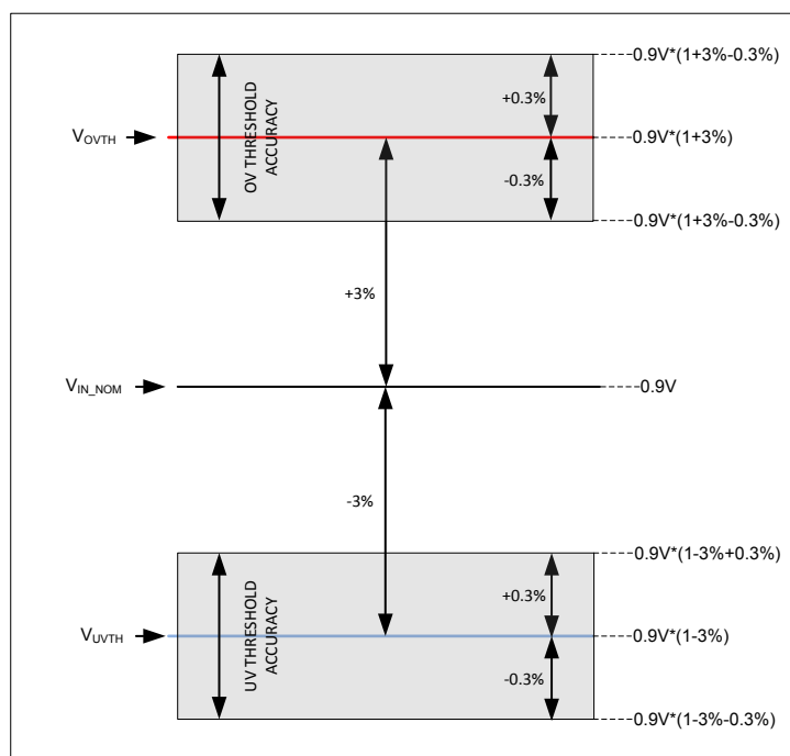
Figure 2. Undervoltage/Overvoltage Threshold Accuracy
