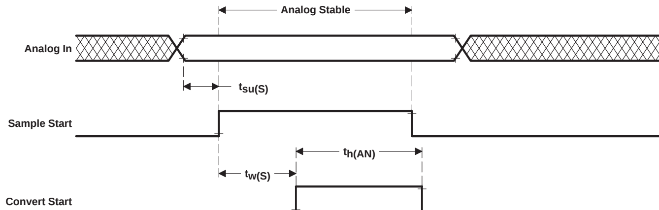
Figure 22. Analog Timing
