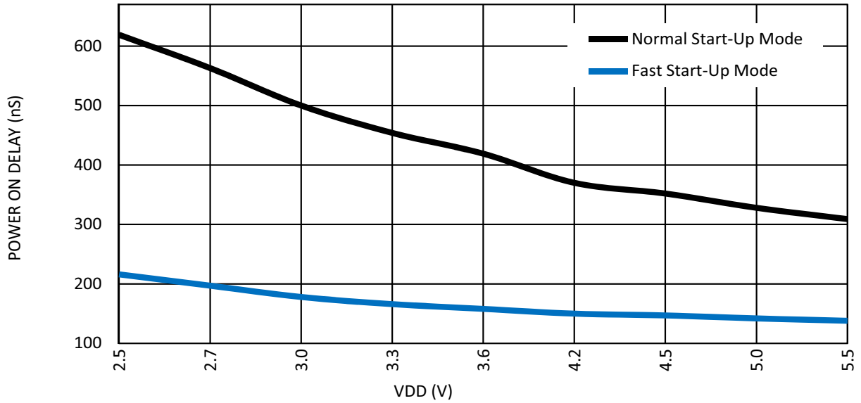
Figure 53: Oscillator Maximum Power-On Delay vs. V_{DD} , T = +25^{\circ}\text{C} , \text{OSC0} = 2\text{ MHz}
