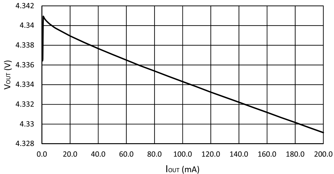
Figure 100: LDO Load Regulation, HIGH POWER Mode, T = 25\text{ }^{\circ}\text{C} , V_{DD} = 5\text{ V} , V_{OUT} = 4.35\text{ V}
