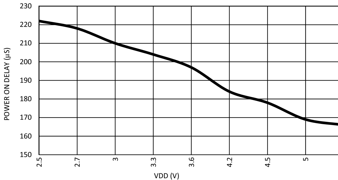
Figure 55: Oscillator Maximum Power-On Delay vs. V_{DD} at T = 25\text{ }^{\circ}\text{C} , \text{OSC1} = 1.73\text{ kHz}
