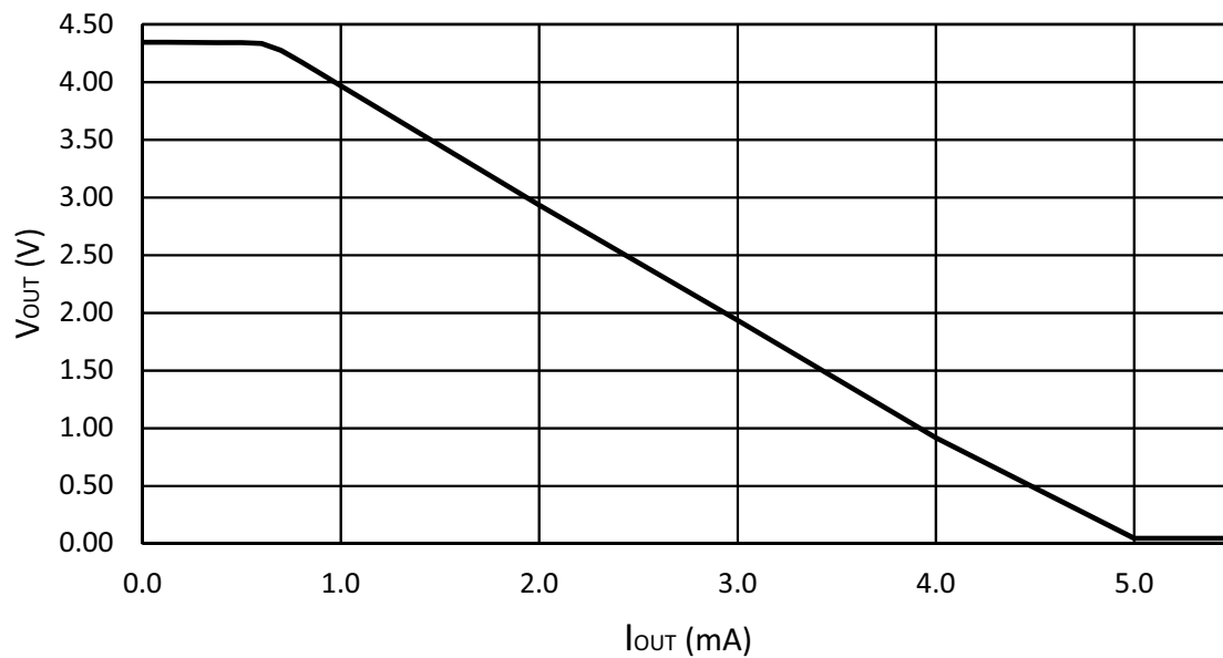
Figure 101: LDO Load Regulation, LOW POWER Mode, T = 25\text{ }^{\circ}\text{C} , V_{DD} = 5\text{ V} , V_{OUT} = 4.35\text{ V}
