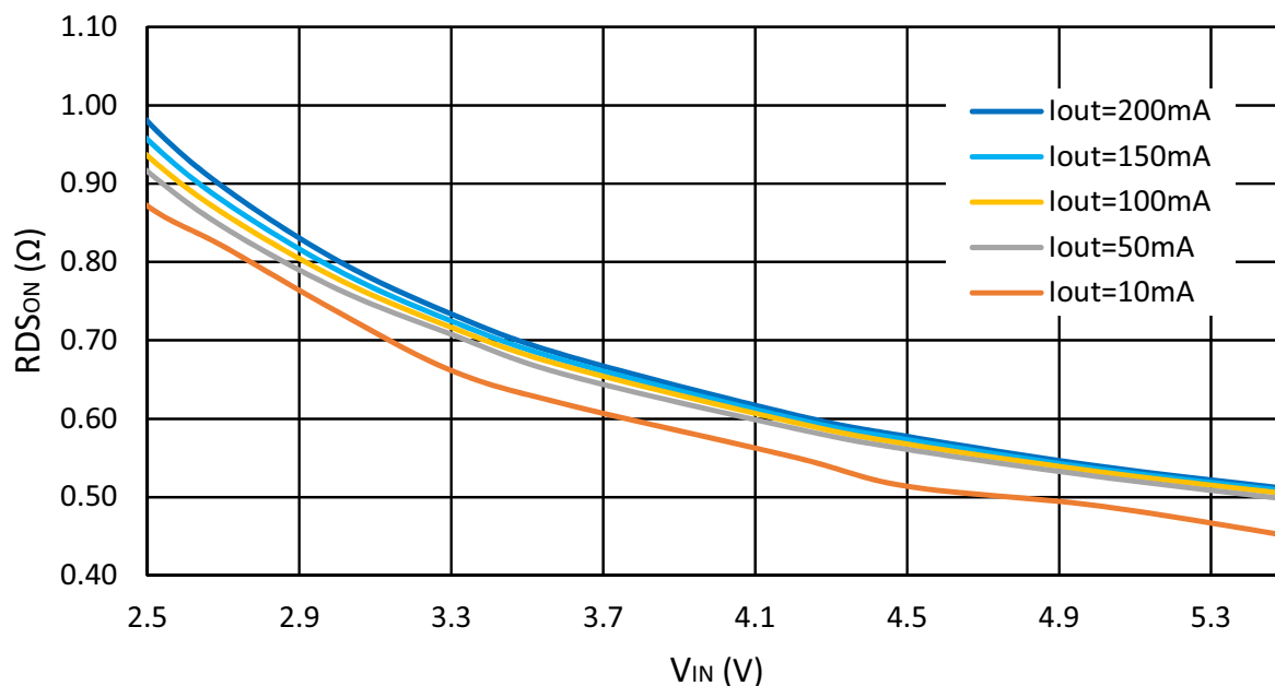
Figure 104: LDO P-Channel ON Resistance R_{DS(on)} vs. V_{IN} , Power Switch Mode, T = 25^{\circ}\text{C}
