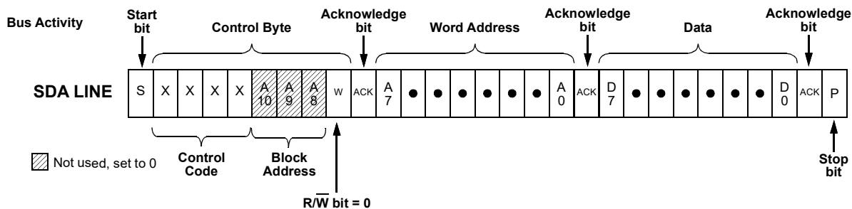
Figure 89: Byte Write Command, R/\bar{W} = 0
