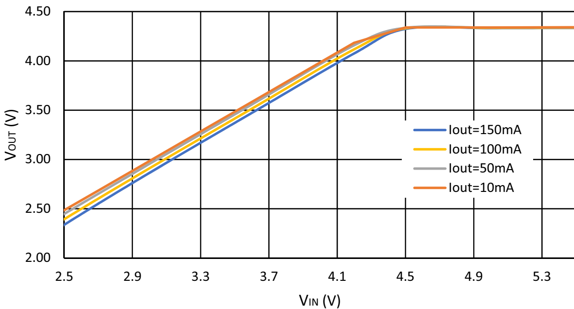
Figure 103: LDO High Power Mode VOUT vs. VIN, T = 25 °C, VDD = 5 V
