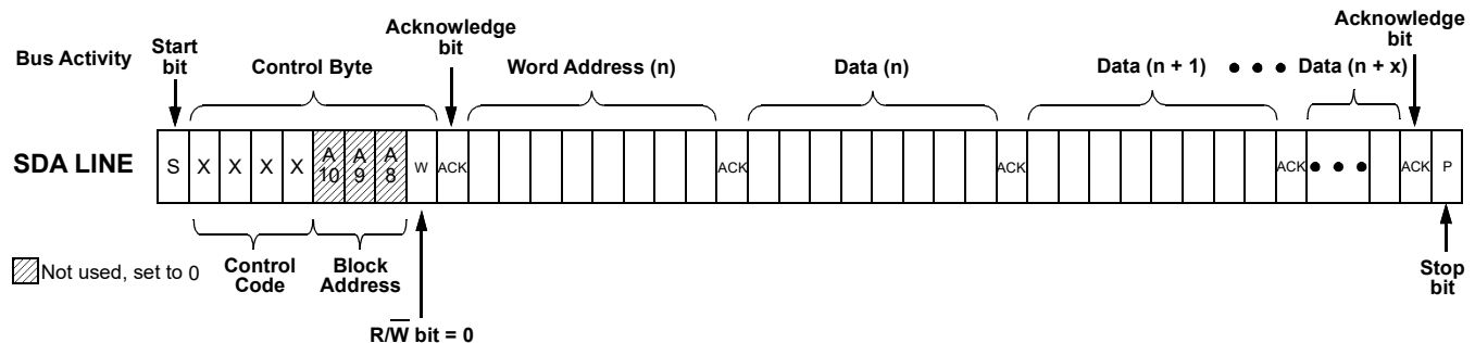
Figure 90: Sequential Write Command, R/\bar{W} = 0
