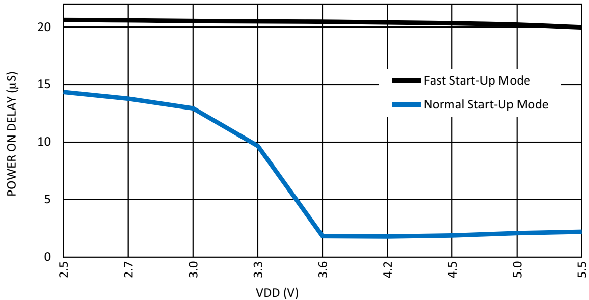
Figure 54: Oscillator Maximum Power-On Delay vs. V_{DD} at T = 25\text{ }^{\circ}\text{C} , \text{OSC0} = 25\text{ kHz}
