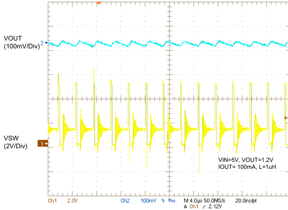
Figure 126: Output Ripple vs. I_{OUT} = 100\text{ mA}
