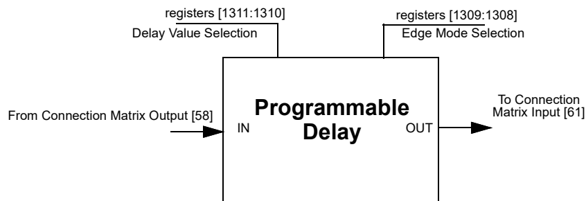
Figure 44: Programmable Delay
