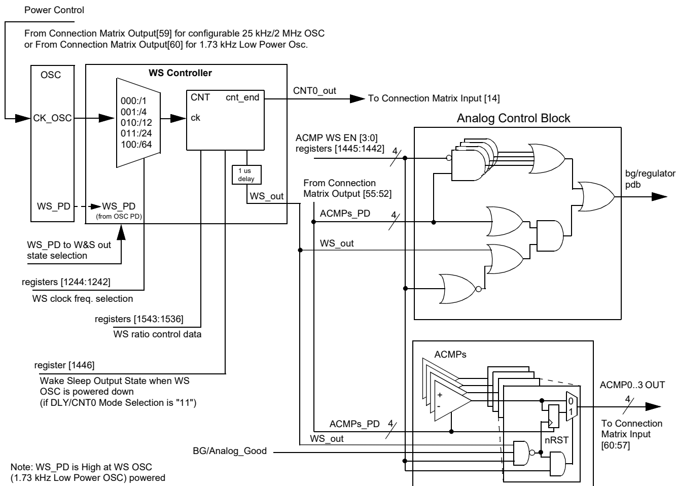
Figure 36: Wake/Sleep Controller
