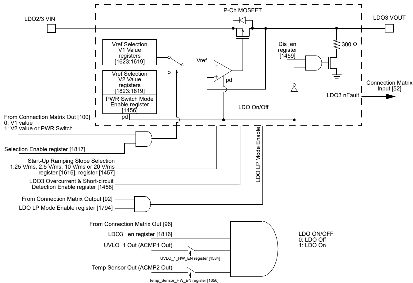
Figure 98: LDO3 Regulator Block Diagram
