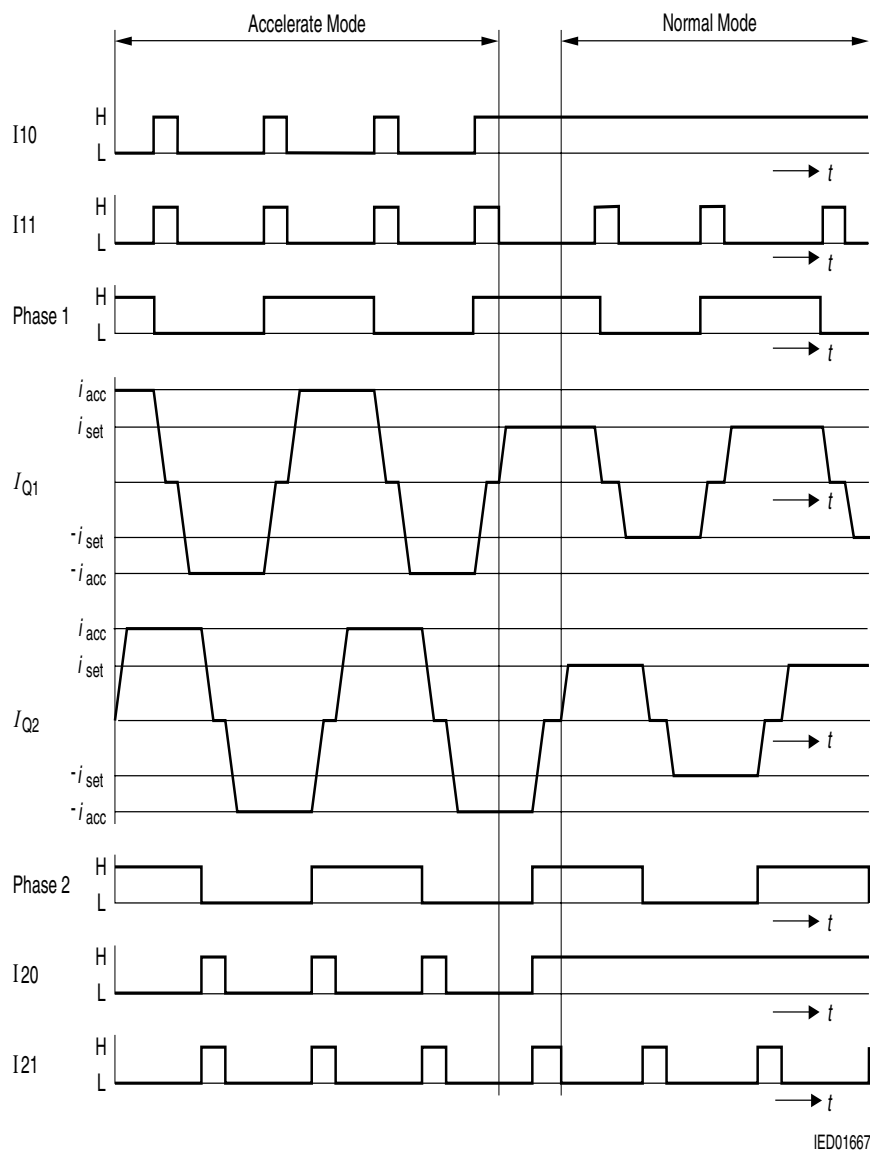
Figure 6 Half-Step Operation
