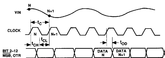
Figure 1. Timing Diagram
