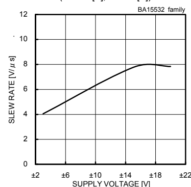
Fig. 260 Slew Rate - Supply Voltage ( C_L=100[pF] , R_L=2[k\Omega] , T_a=25[^\circ C] )
