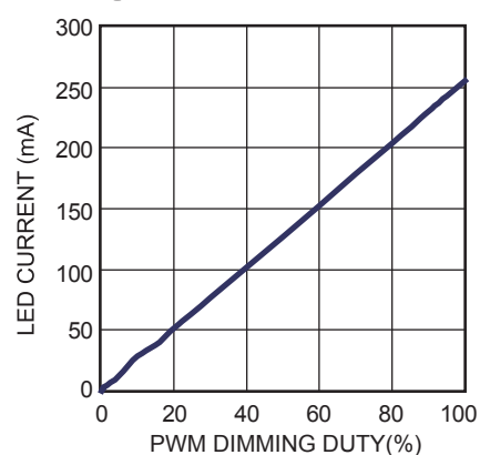
PWM Dimming Linearity @ 200Hz
