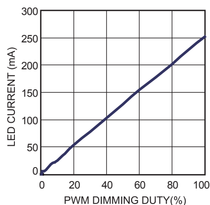
PWM Dimming Linearity @ 2kHz
