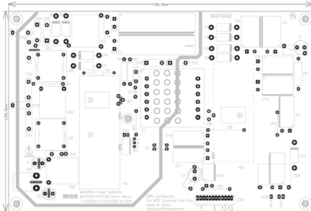
Figure 6: Top Layer
