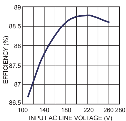
System Efficiency
