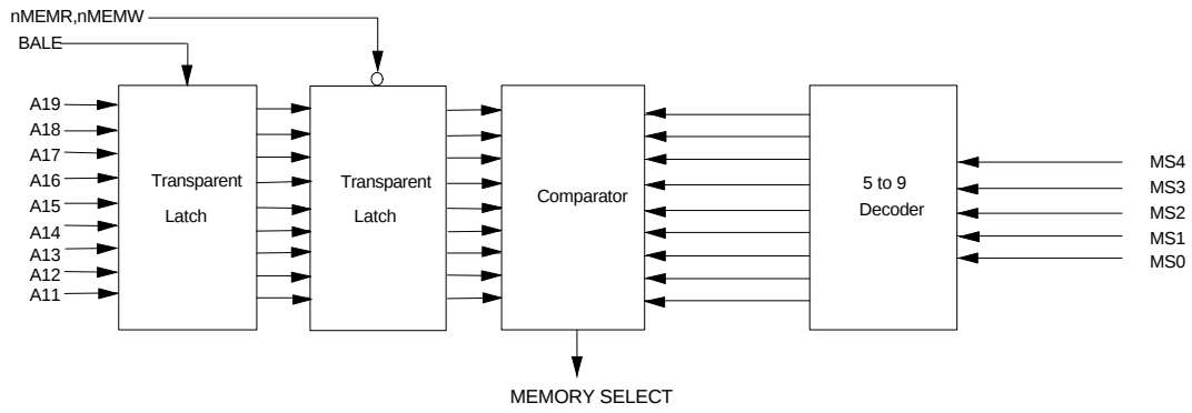
FIGURE 4 - MEMORY SELECTOR
