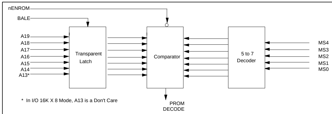
FIGURE 5 – PROM SELECTOR
