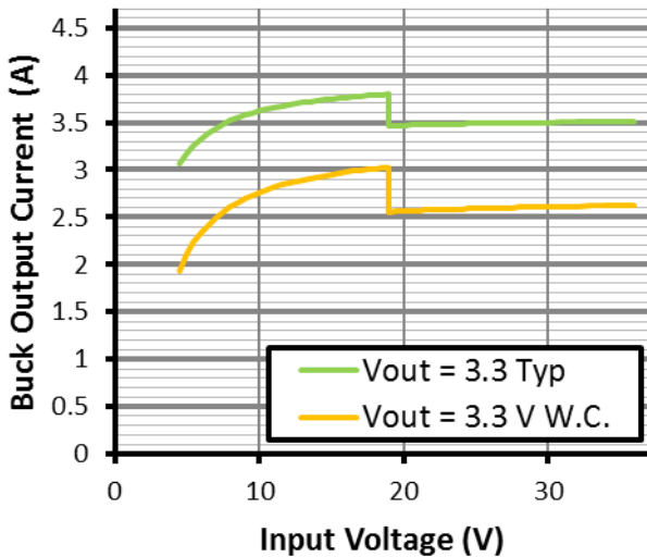
Figure 42. Switcher 1 Dc Output Current vs. VIN with a 2.2 \mu\text{H} Inductor
