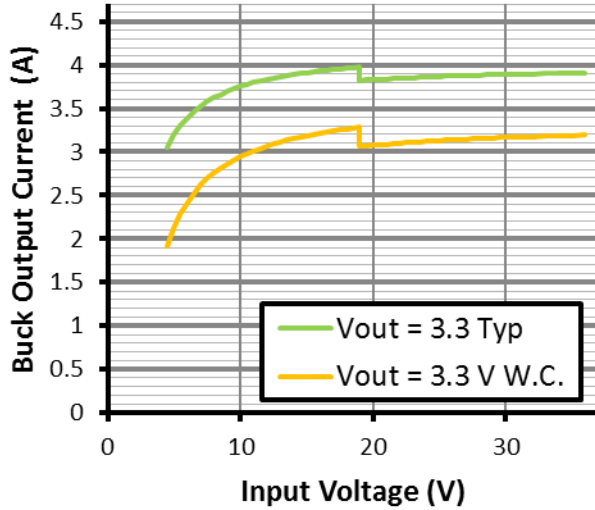
Figure 41. Switcher 1 Dc Output Current vs. VIN with a 4.7 \mu\text{H} Inductor
