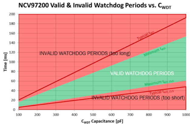
Figure 37. NCV97200 Valid & Invalid Watchdog Periods vs. C_{WDT}
