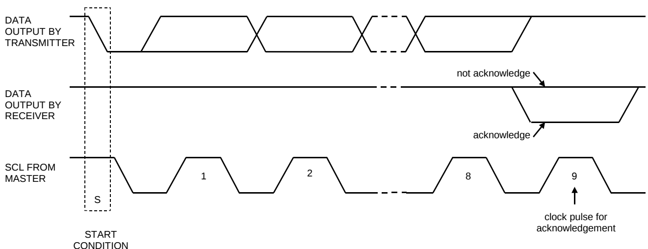
Figure 31. Acknowledge (I²C-bus)
