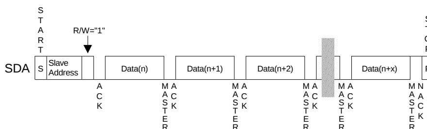
Figure 28. Data Transfer Sequence in I²C-bus Mode
