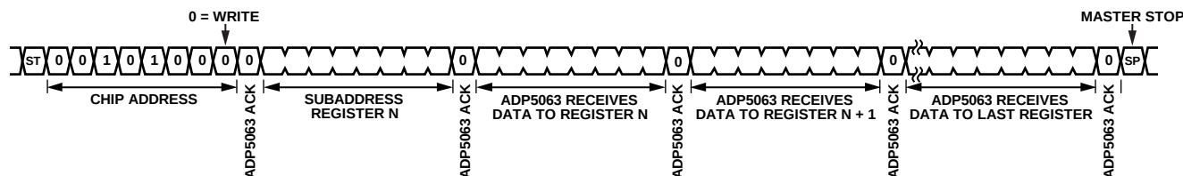
Figure 32. I 2 C Multiple Register Write Sequence
