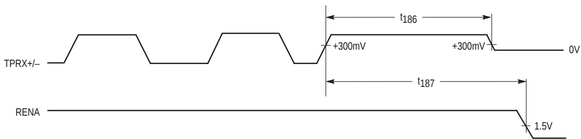
Figure 33. RENA Deassertion Delay from Last Valid Positive Transition of TPRX Pair
