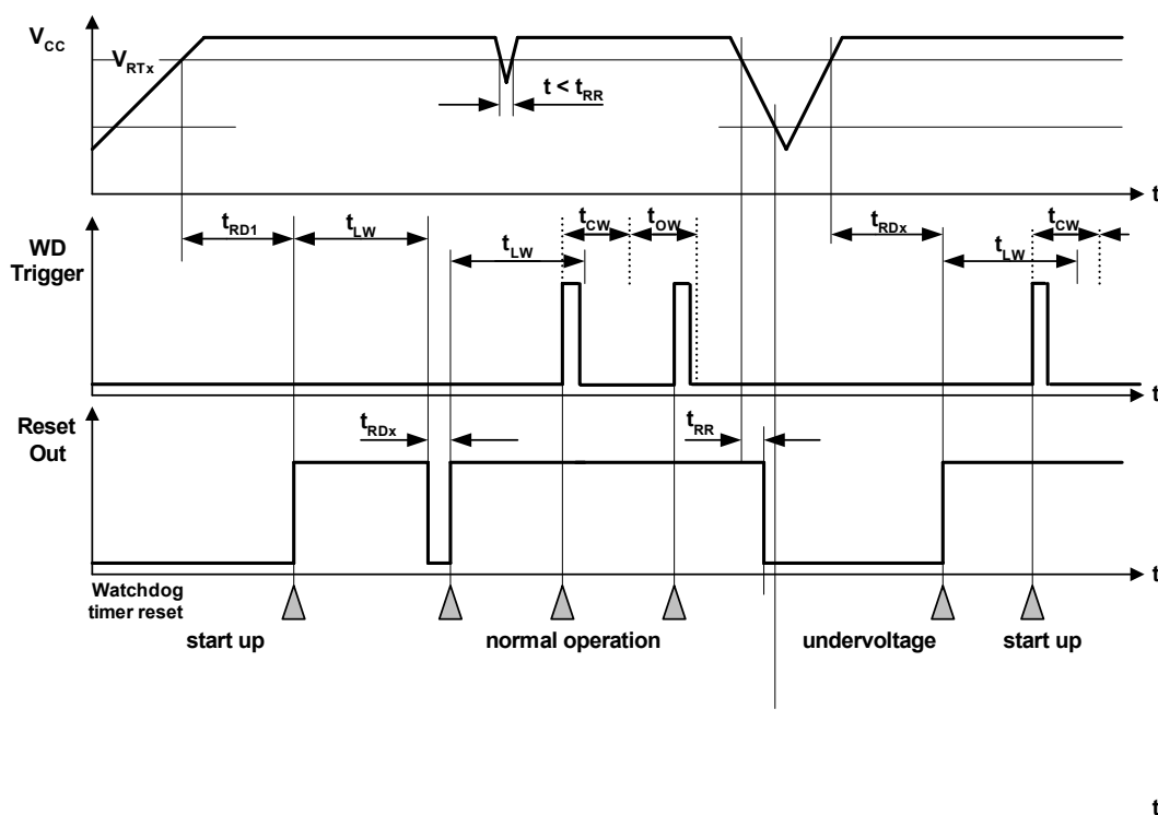
Figure 17 Reset Timing Diagram
