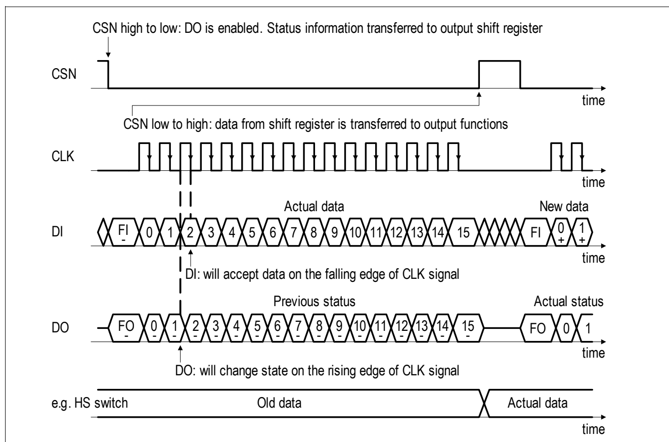
Figure 13 SPI-Data Transfer Timing
