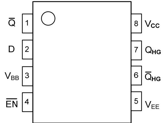
CTS100EL100VOTG (MSOP8)
