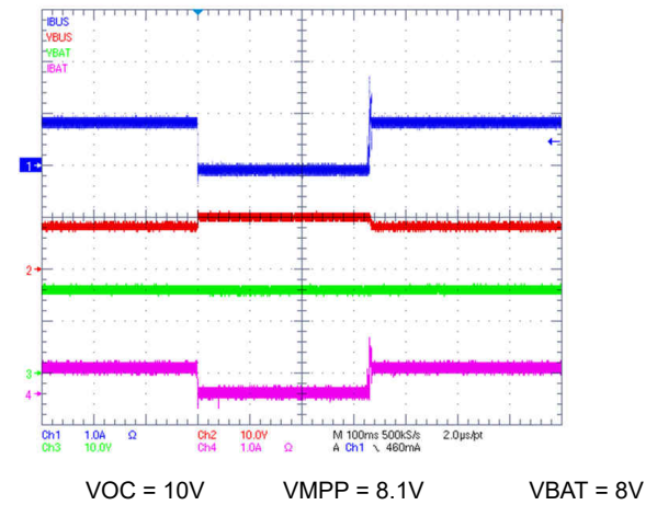
Figure 10-19. MPPT Operation Zoom
