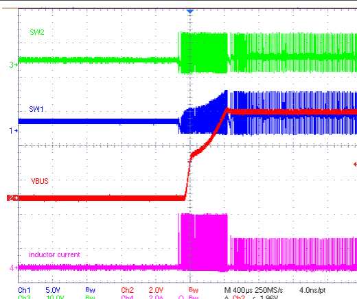
Figure 10-11. Buck Mode PFM with OOA
