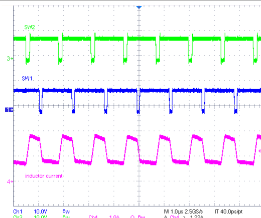
Figure 10-9. Buck-Boost Charging Mode PWM Operation
