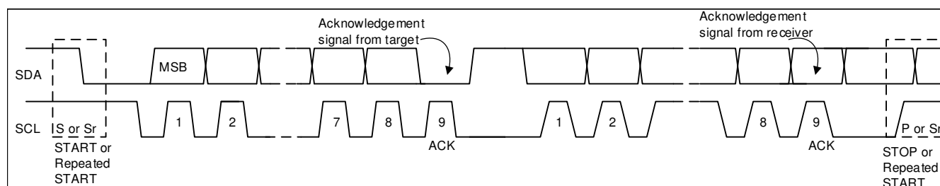
Figure 9-18. Data Transfer on the I²C Bus
