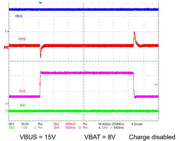
Figure 10-15. VSYS Load Transient Response
