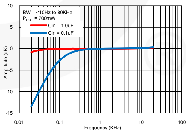
Figure 15. Frequency Response
