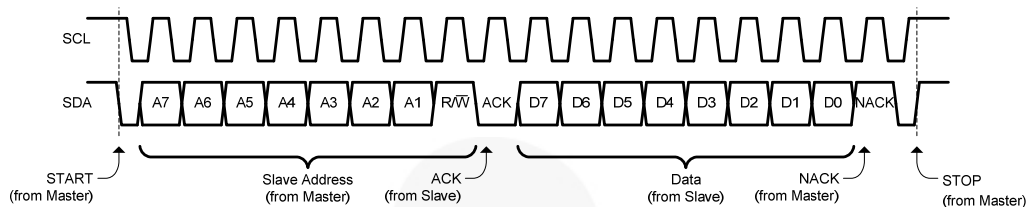
Figure 29. I²C Read
