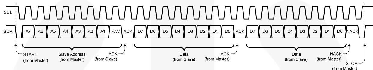
Figure 30. I²C Multiple Byte Read
