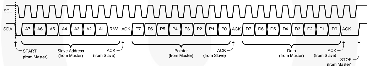
Figure 31. I²C Write
