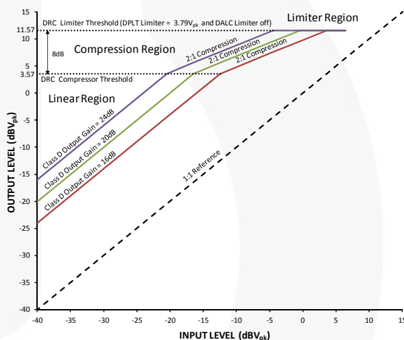
Figure 25. Dynamic Range Compression Response vs. Class-D Output Gain Settings
