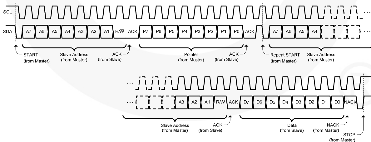
Figure 32. I²C Write Followed by Read
