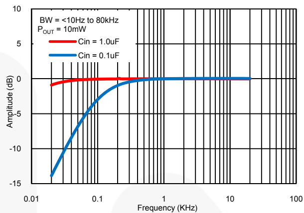
Figure 22. Frequency Response
