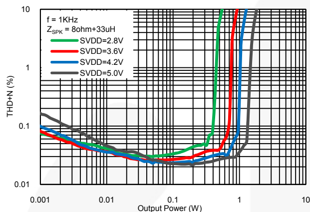
Figure 10. THD+N vs. Output Power
