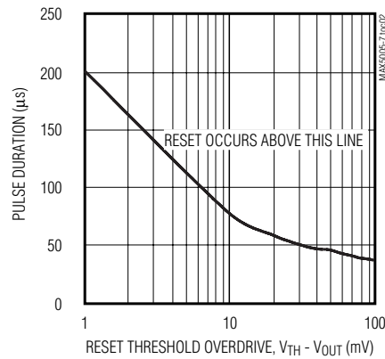
MAXIMUM PULSE DURATION vs. RESET THRESHOLD OVERDRIVE
