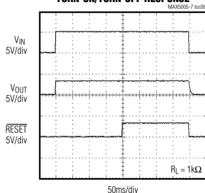
TURN-ON/TURN-OFF RESPONSE
