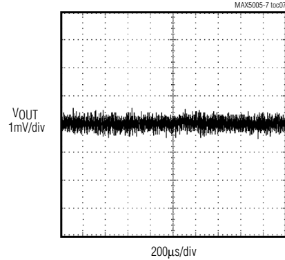
OUTPUT NOISE
