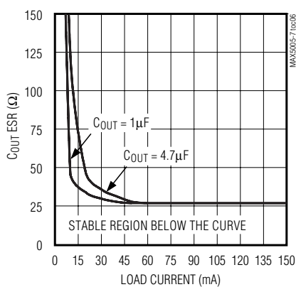
REGION OF STABLE C_{\text{OUT}} ESR vs. LOAD CURRENT
