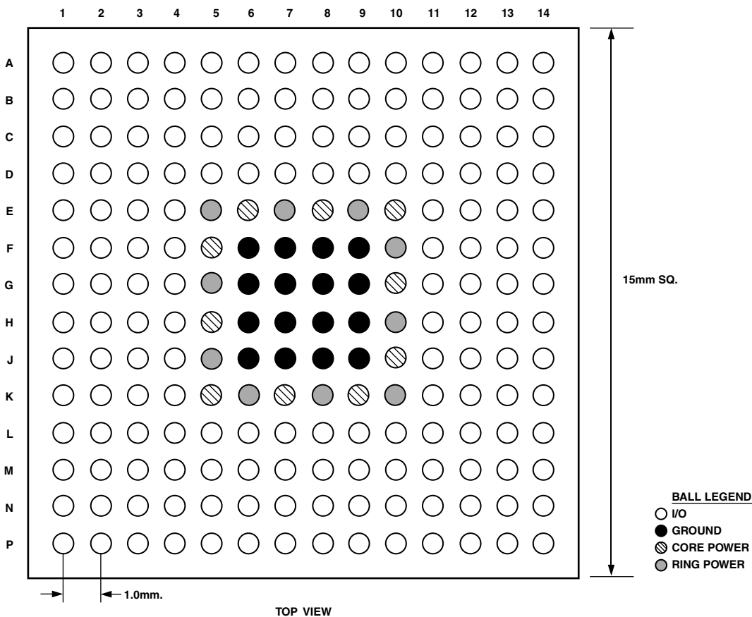
PIN CONFIGURATION (Top View)
