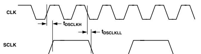
Figure 6. SCLK Switching Characteristic (Divide by 3 or ODD Integer)
