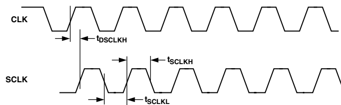
Figure 4. SCLK Switching Characteristics (Divide by 1)
