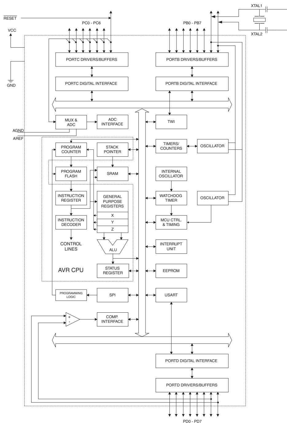
Figure 2-1. Block Diagram
