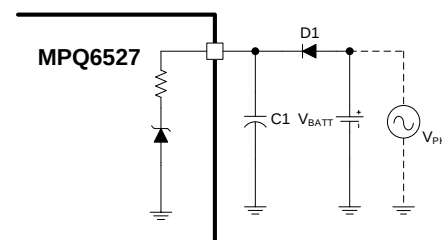
Figure 5: Discharger Circuit Functional Principle
