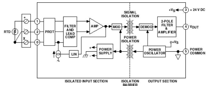
Figure 1. 7B34 Functional Block Diagram
