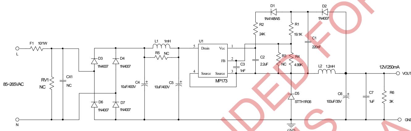
Figure 9—Typical application at 12 V, 250 mA
