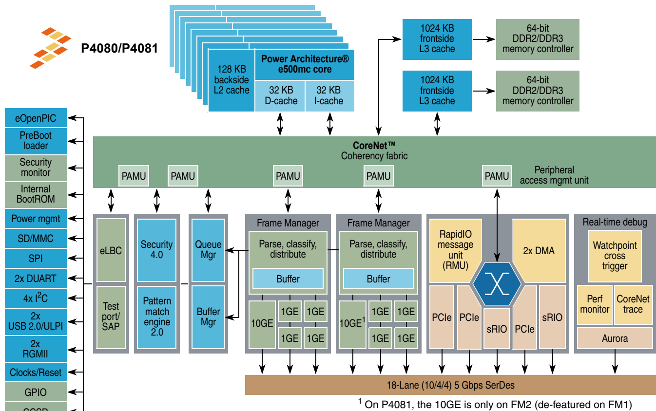
Figure 1. P4080/P4081 QorIQ Preliminary Block Diagram
