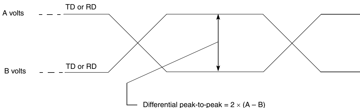
Figure 43. Differential Peak-Peak Voltage of Transmitter or Receiver
