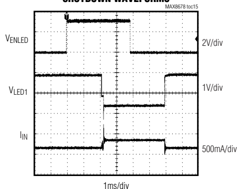
LED STARTUP/ SHUTDOWN WAVEFORMS
